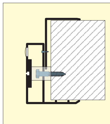
3. PK3 aluminium Lining 130-170 mm
